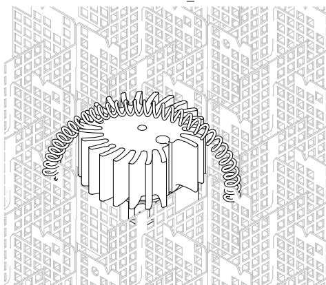
Top view PUNTEO-N 1x1 S07 in TICELL_N 33.64H40
