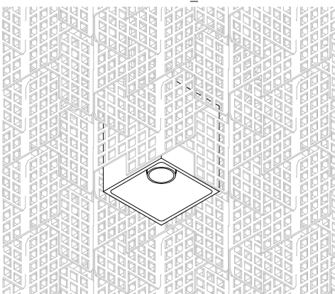
Bottom view PUNTEO-N 1x1 S07 in TICELL_N 33.64H40
